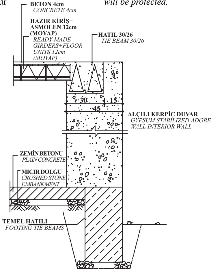
Şekil 3.11 Sistem Kesiti Figure 3.11. Cross-Section of the System
